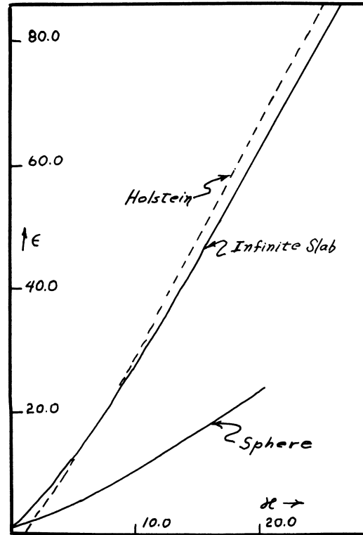
FIG. 1. Display of \epsilon as a function of \kappa . Solid lines—this paper; dashed lines—Holstein's approximation [Eq. (4.1)].
